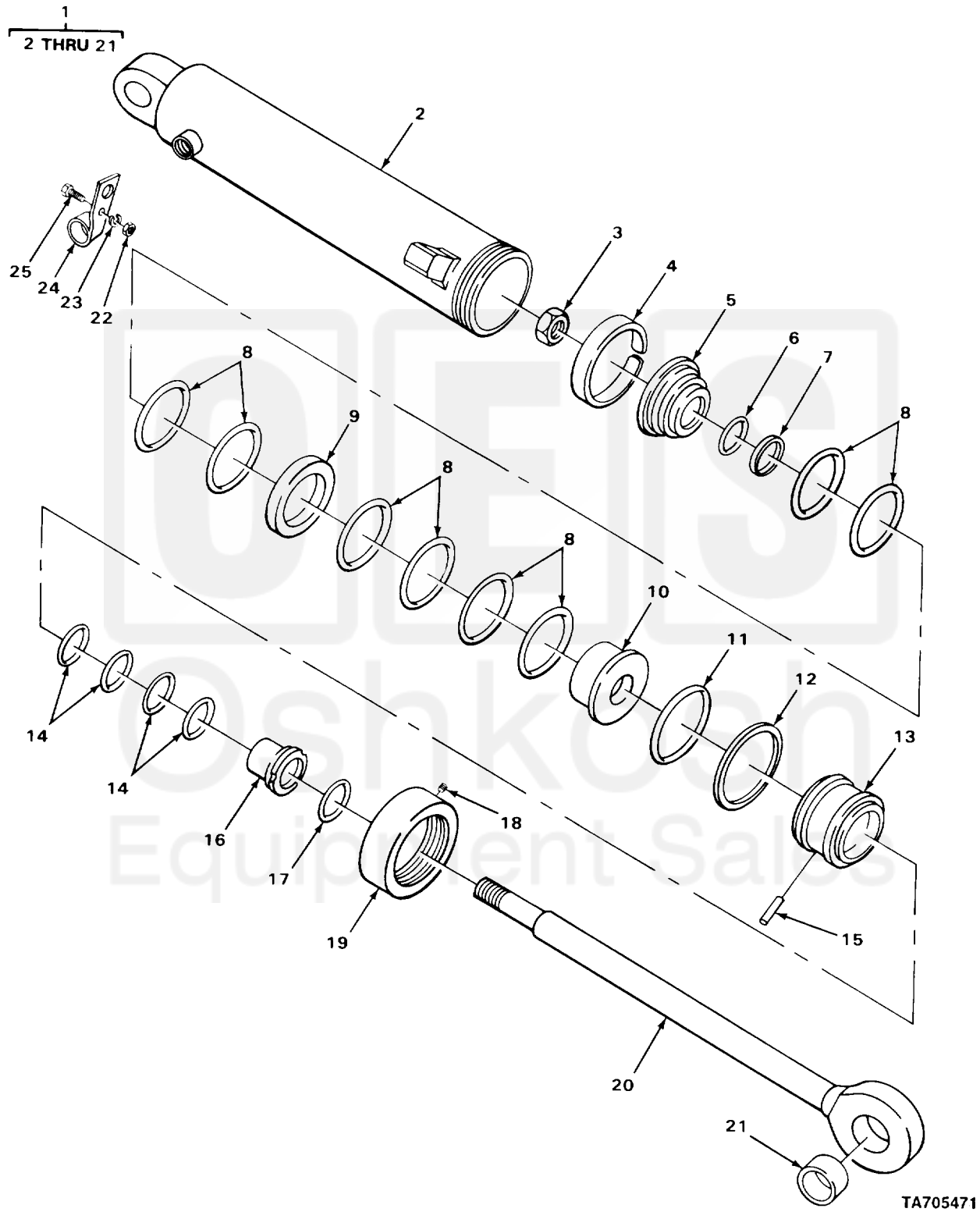
FIGURE 145. STEERING CYLINDER (MHE-200 AND MHE-222).
